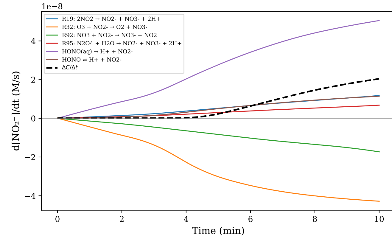
(c) \text{NO}_2^-
