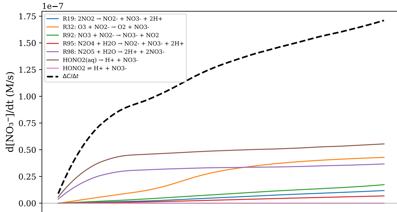
(a) \text{NO}_3^-
