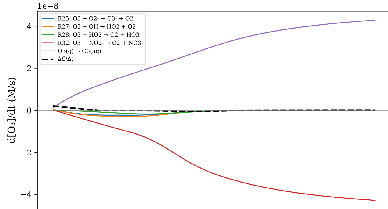
(b) \text{O}_3
